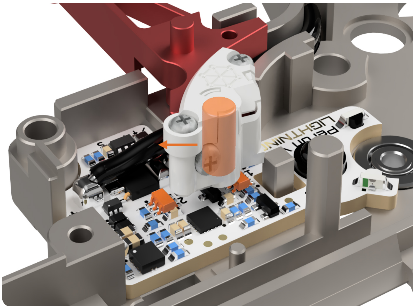
Trigger position sensing
