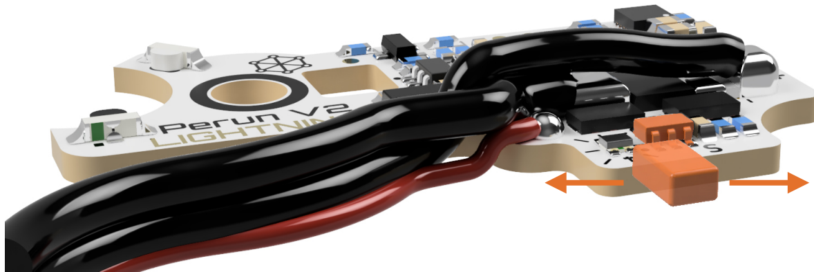
Selector plate position sensing
