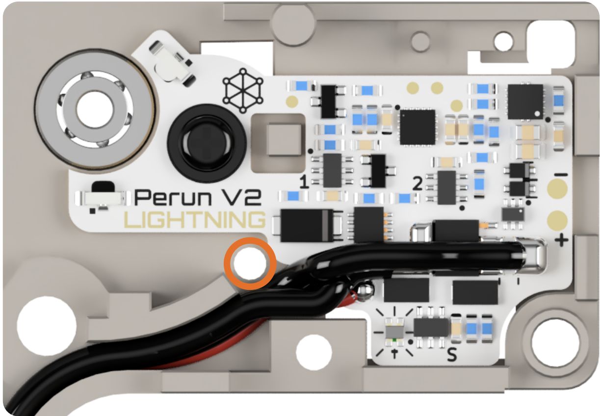
Correct wire channeling in the back wired variant. Make sure wires do not cover the hole for the middle pin!
