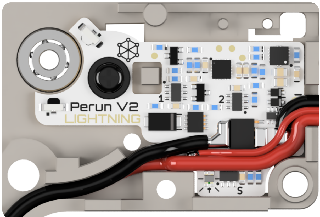
Correct wire channeling in the front wired variant.
